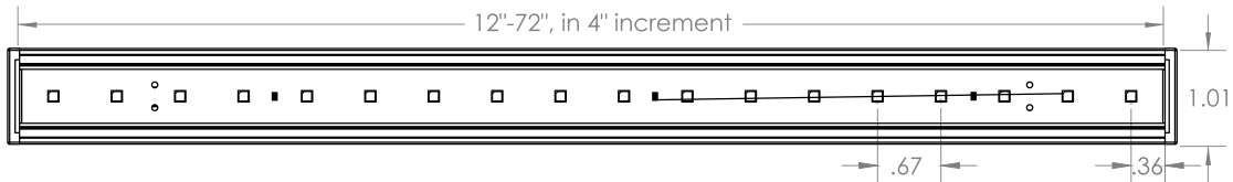
1 PLAN VIEW
