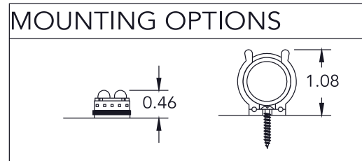
MOUNTING TAPE TUBE (using approved adhesive tape fixture can rotate in tube)
