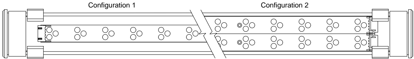
2 PLAN VIEW [CCS-100] SCALE: 6"=1'-0"
