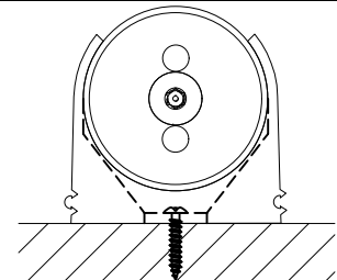
FIXED TUBE- FIXTURE CAN ROTATE IN TUBE
