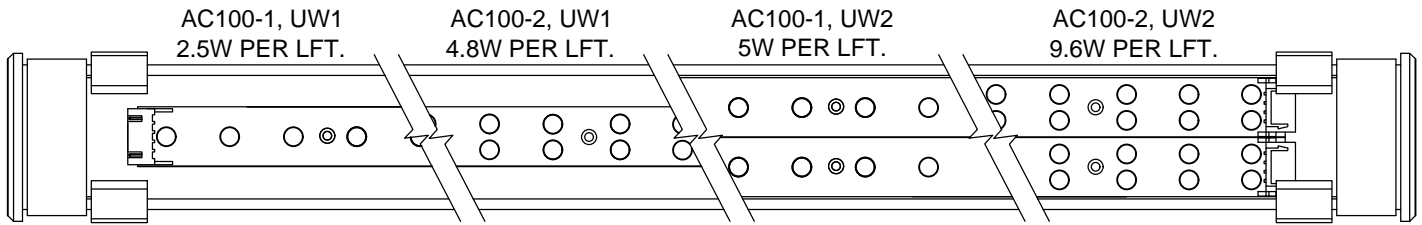
1 PLAN VIEW [AC-100] SCALE: 6"=1'-0"
