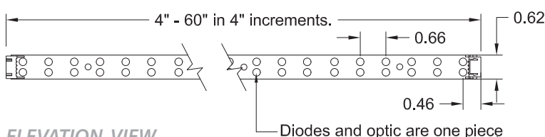
ELEVATION VIEW
